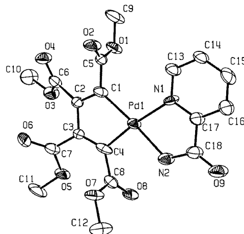
Figure 5. Structure of the [\text{Pd}\{\text{C}_4(\text{COOMe})_4\}(2\text{-HNCOpy})]^- anion in the single crystal structure of 27 . All hydrogen atoms have been omitted for clarity.
