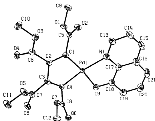
Figure 3. An ORTEP representation of 13 .
