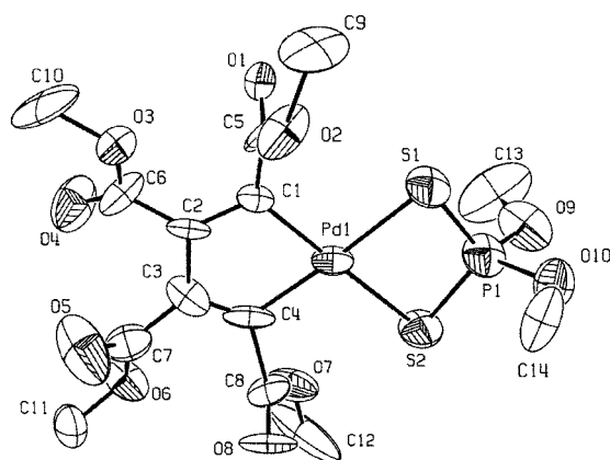
Figure 4. ORTEP diagram of 20 ; thermal ellipsoids are drawn at the 50% probability level.
