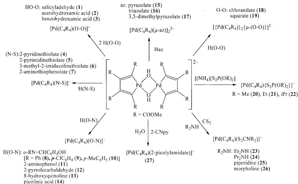
Scheme 1. Reactivity of the hydroxo complex [\text{NBu}_4]_2[\text{Pd}_2\{\text{C}_4(\text{COOMe})_4\}_2(\mu\text{-OH})_2] ( I ).
