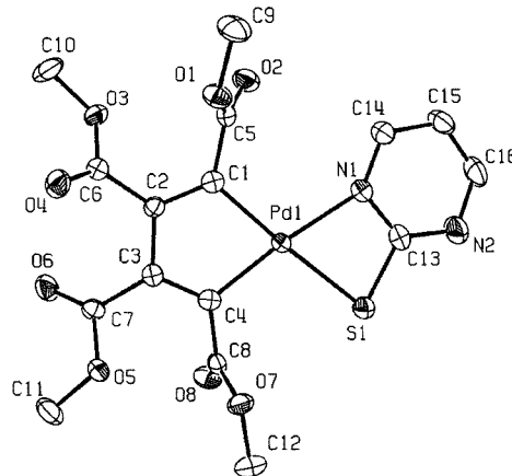
Figure 1. ORTEP diagram of anion complex 5 with the atom numbering Scheme; thermal spheres are drawn at the 50% probability level.
